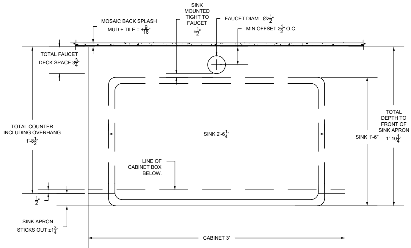
MARON SINK DETAIL 1-1/2" = 1'-0"
